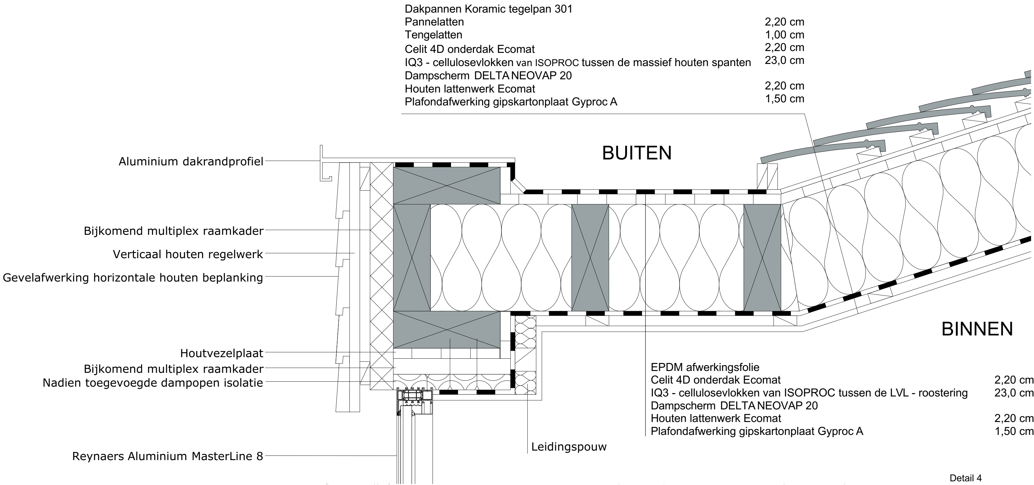
Detail 4
